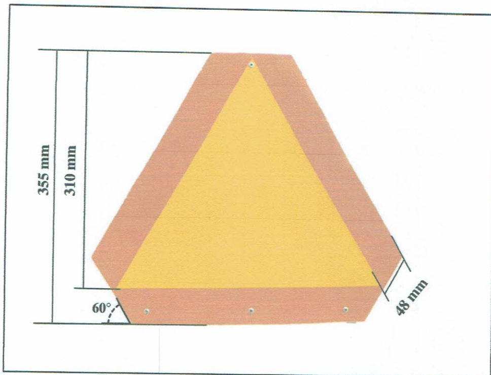
Figure 2. Dimensions of the SMV Emblem.
