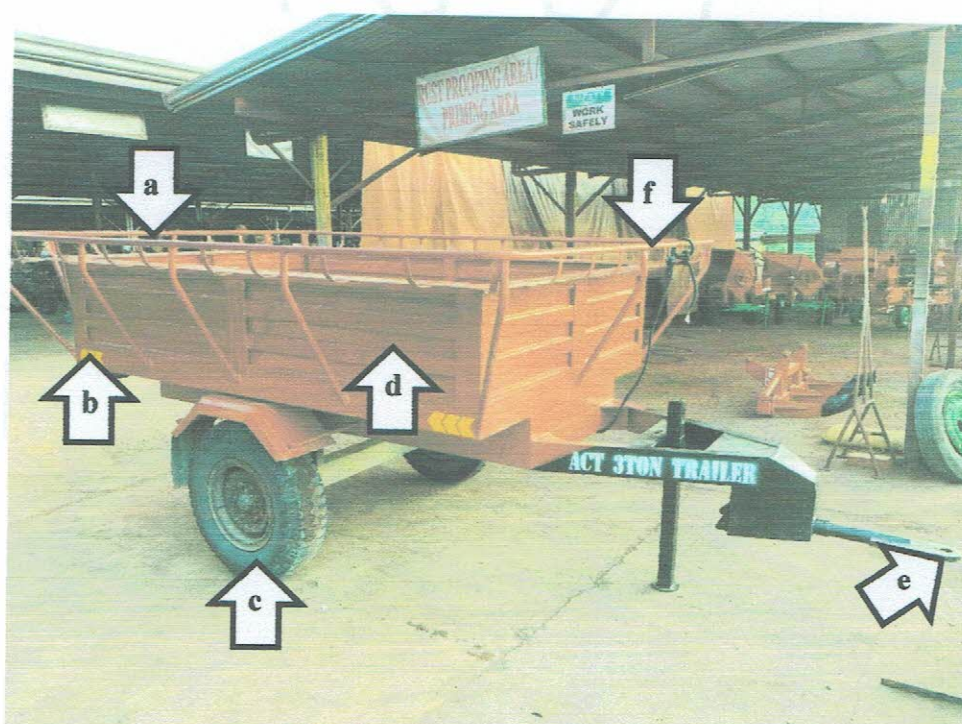
Figure 1. Parts of the ACT 3 TONNE TRAILER Agricultural Trailer hitched to 70.8 kW MASSEY FERGUSON 5709 Four-wheel Tractor includes the following: (a) Loading platform, (b) Yellow reflector, (c) Transport wheels, (d) Sideboard, (e) Hitch point, and (f) Extension for loading.
